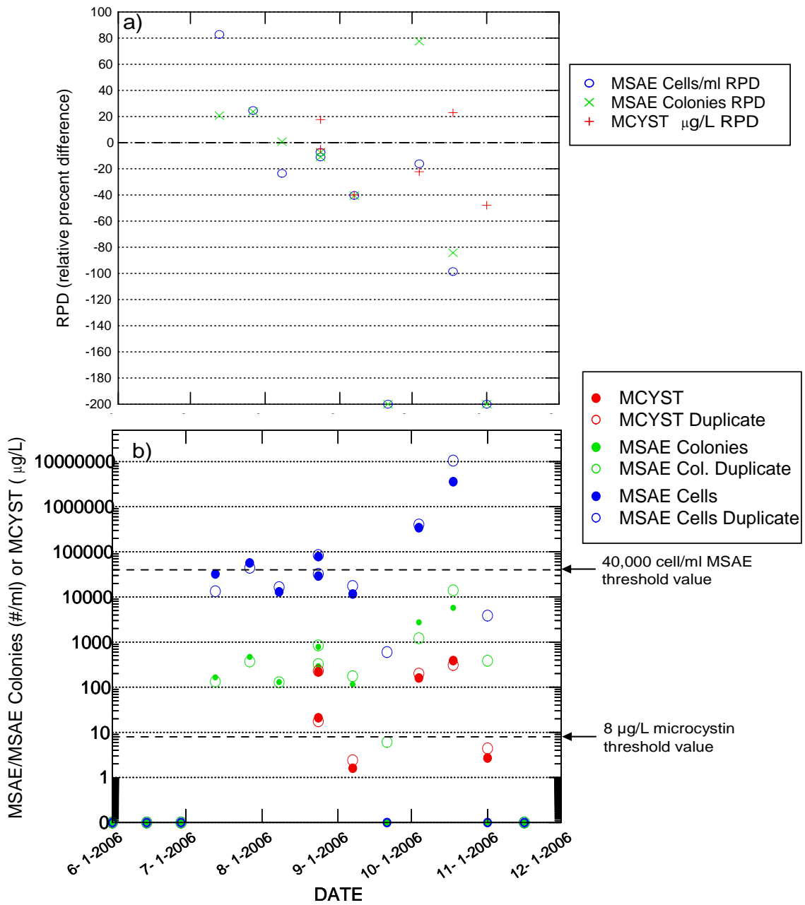
Figure 2. Analysis of field duplicate samples for MSAE cell density and microcystin concentration (MCYST); relative percent difference (RPD) (a), and paired sample values (b).
