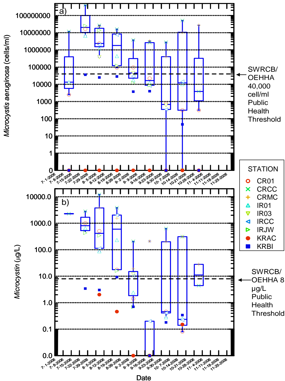
Figure 3. Time-series of MSAE cell density (a) and microcystin toxin concentration (b) for Copco and Iron Gate Reservoir stations, 2006. The blue box is for the reservoir stations only; the river stations KRAC and KRBI are shown independently.
