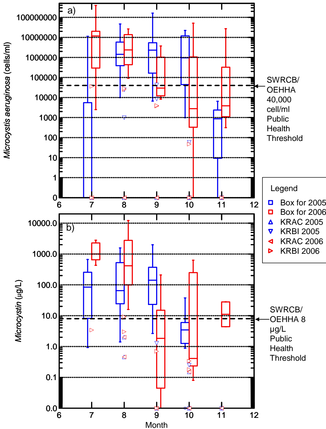
Figure 8. MSAE cell density (a) and microcystin toxin concentration (b) compared between 2005 and 2006.
