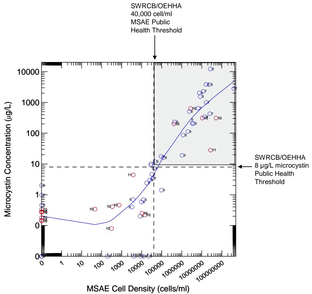
Figure 6. Relationship between MSAE cell density and microcystin toxin concentration (symbol labels are sample dates and October-November dates are shown in red); shown with distance weighted least squares (DWLS) smoother applied to all data, Copco and Iron Gate Reservoirs, 2005.
