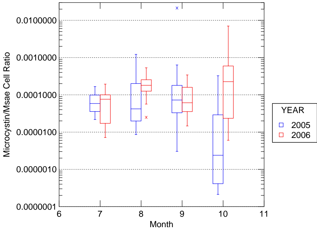
Figure 7. Box plot of the ratio of microcystin toxin per unit MSAE cell density for Copco and Iron Gate Reservoirs, 2005 and 2006. Lower hinge of the box is the lower quartile (25 th percentile), upper hinge is the upper quartile (75 th percentile), and the whiskers are values 1.5x the upper or lower quartile.
