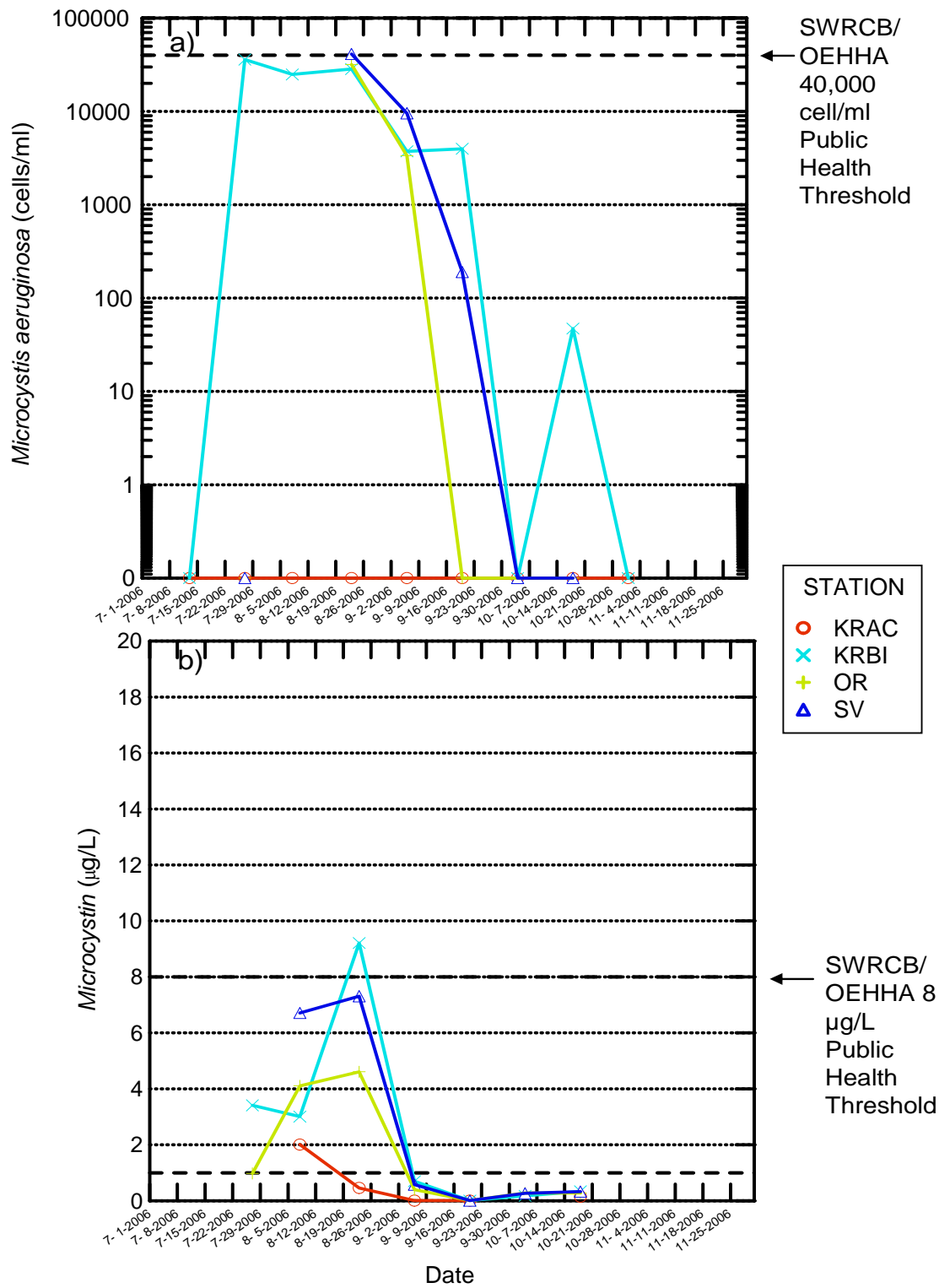
Figure 4. Time-series of MSAE cell density (a) and microcystin toxin concentration (b) for Klamath River Stations KRAC, KRBI, SV, and OR, 2006
